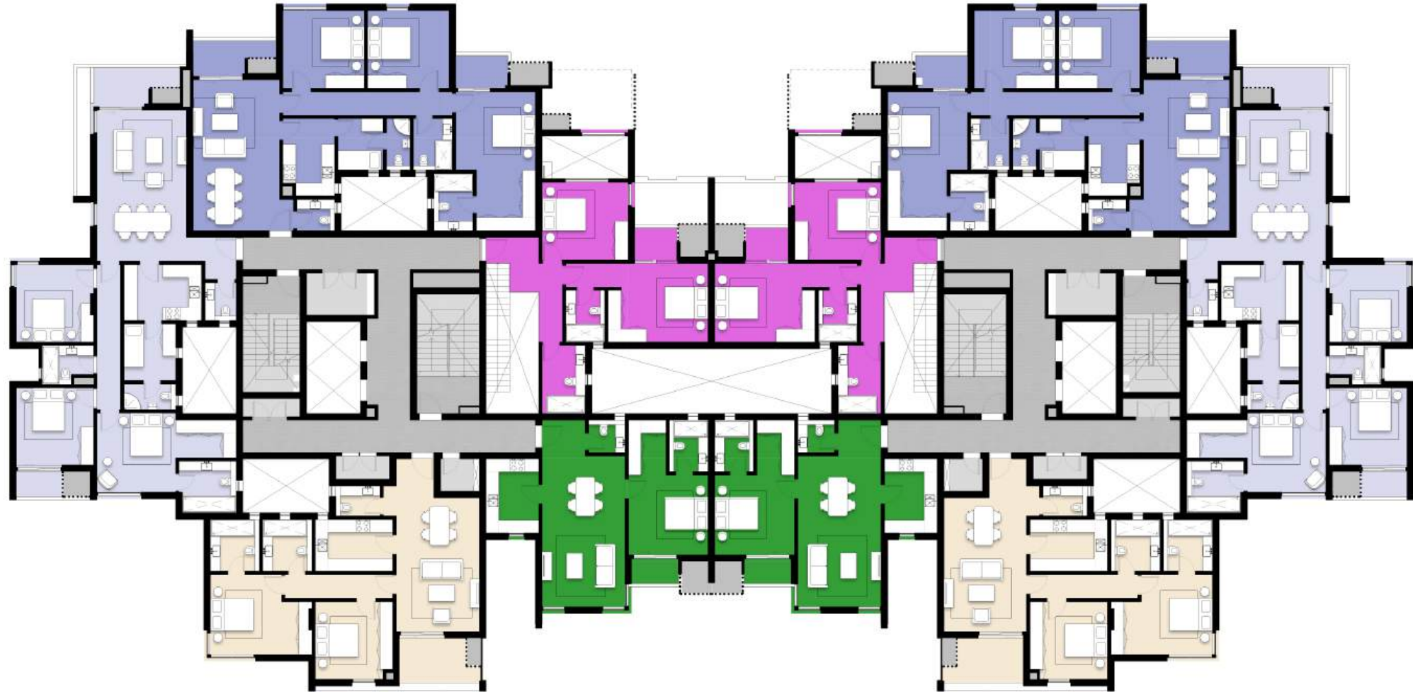
Third Floor
